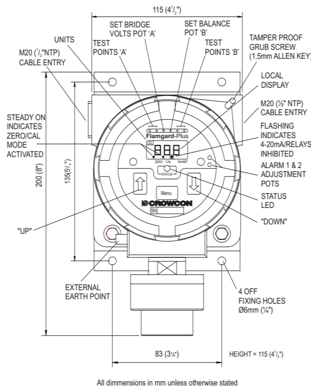
Diagram 1: Flamgard Plus general arrangement
