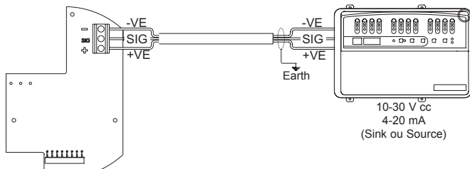
Diagram 5: Xgard IR electrical connections
