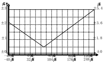
Figure 2 Temperature Accuracy
