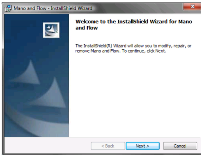
Software installatie-assistent
