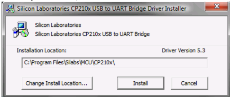
Driver installatie-assistent
